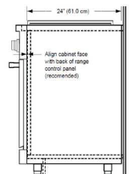
View of Range Installed (Side View)
